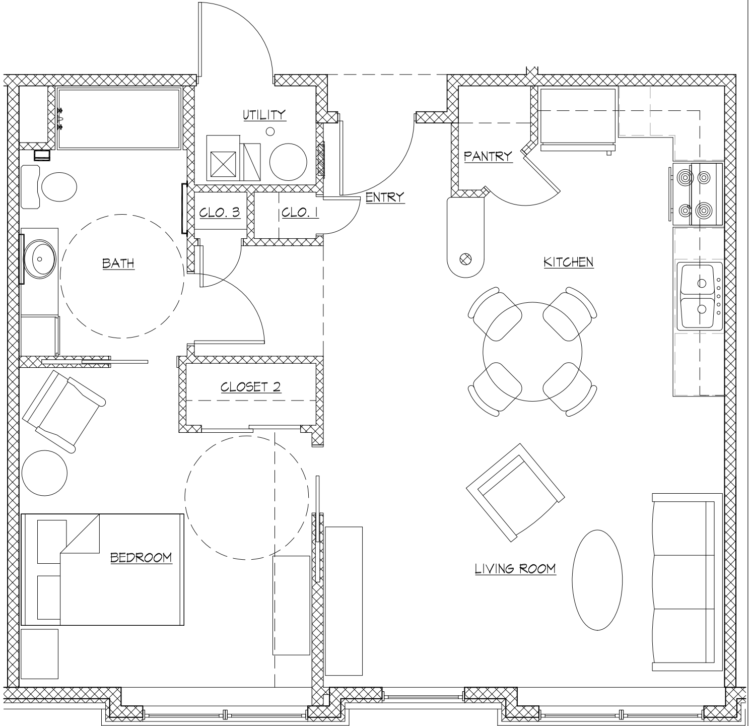
TYPICAL UNIT FLOOR PLAN SCALE: 1/4" = 1'-0"
